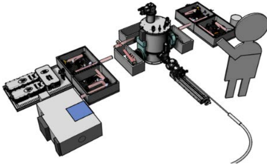
Setup Terahertz / Infrared magneto-ellipsometer
