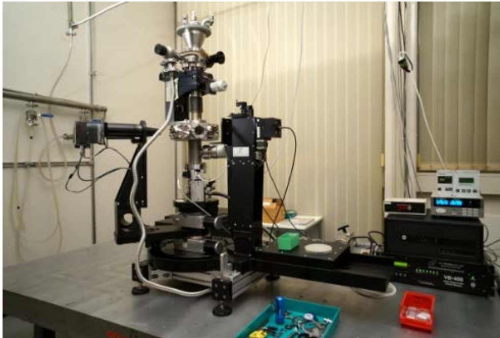
Setup Visible Ellipsometer
