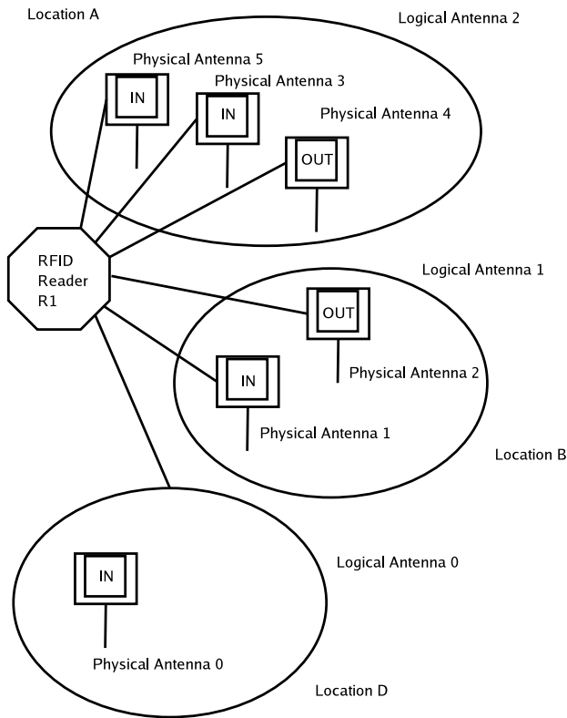
Fig. 16. Schematic view of a reader's settings.
