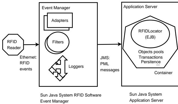
Fig. 10. The Event Manager and the Application Server.
