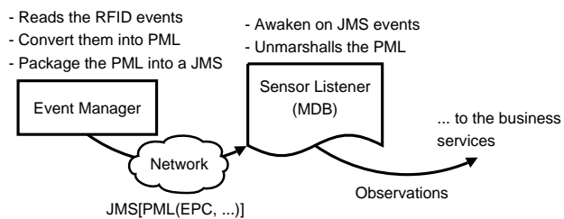
Fig. 13. Asynchronous communication between the EM and the application.
