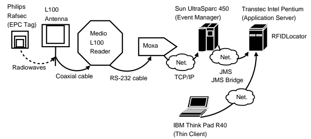
Fig. 18. The hardware devices of our configuration.
