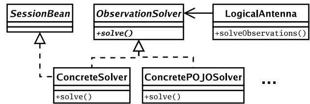
Fig. 14. Logical antenna and observation solvers.
