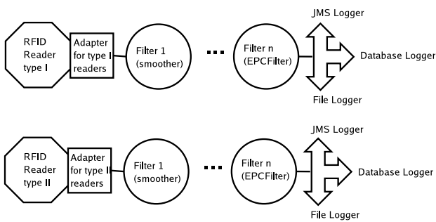
Fig. 6. An example of modules combination in the EM.
