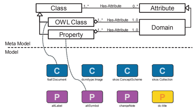
Figure 3: Sample of an Ontology Model and Meta Model
