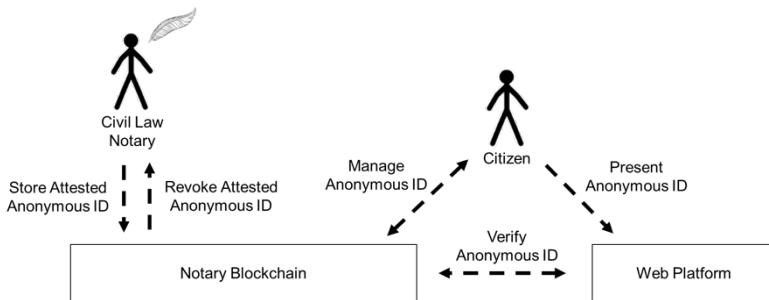
Figure 4: Managing Anonymous IDs Using a Notary Blockchain
