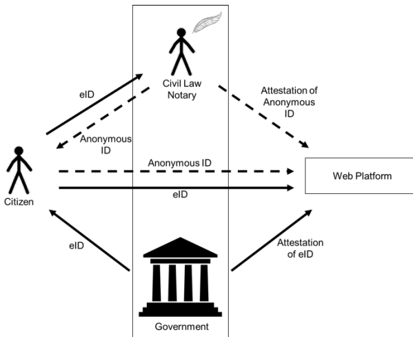
Figure 3: Issuance of Anonymous IDs Through Notaries
