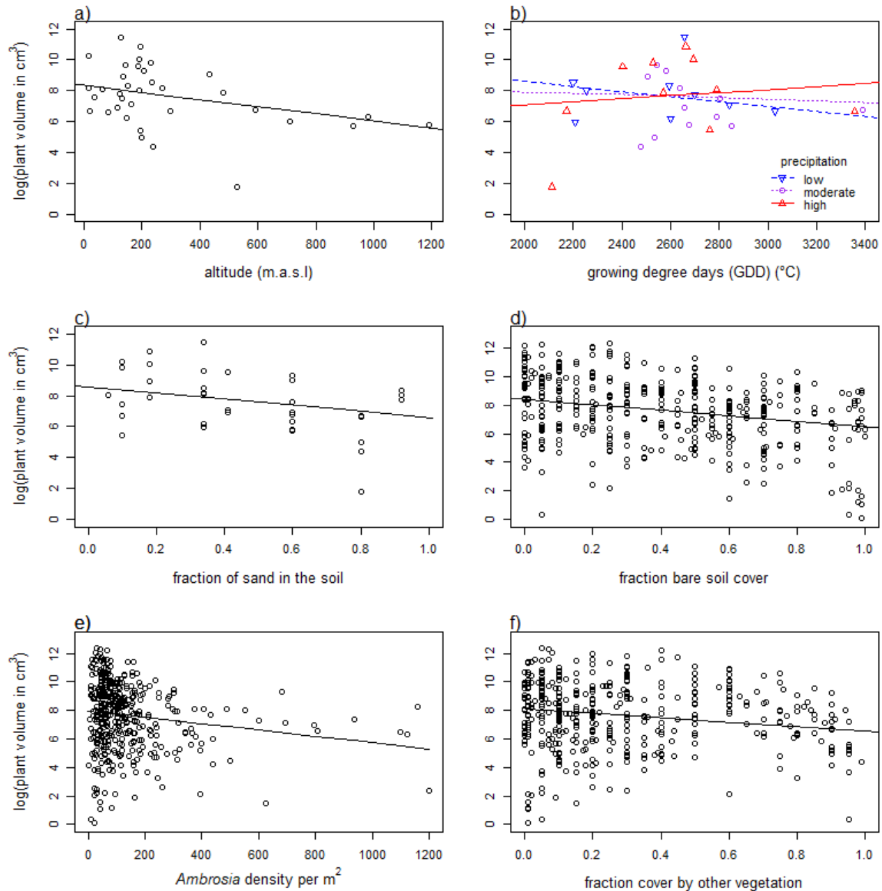
Fig. 3 Effects of different environmental factors on plant volume. Symbols represent observed values per site (a-c) or per plot within sites (d-f) with corresponding fitted regression lines. Panels present the effect of a) altitude, b) the interaction of growing degree days and precipitation (low=<2.2 mm/day, moderate=2.2-2.7 mm/day, high =>2.7 mm/day), c) the fraction of sand in the soil, d) the fraction of bare soil, e) Ambrosia density, and f) the fraction of soil in the plot covered by vegetation other than Ambrosia .
