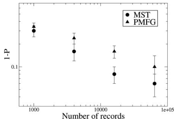
Fig. 3. Analysis of stability of the MST and PMFG with respect to the statistical uncertainty present in the estimation of the correlation matrix as a function of the number of records of the multivariate time series. By assuming as reference matrix the empirical correlation matrix of the system, we perform 4 sets of 20 realizations, each one of surrogated multivariate time series. Each set is characterized by a different number of records set as follows: 1,000, 4,000, 16,000, and 64,000 records. For each of the simulated realizations, both the MST and PMFG have been constructed. The percent ( 1 - P ) of the number of links of the simulated graphs nonmatching with the links of the MST and PMFG of real data are shown as a function of the number of records of the surrogated time series in a log-log plot. (The error bar indicates one standard deviation of 1 - P computed for each set.)
